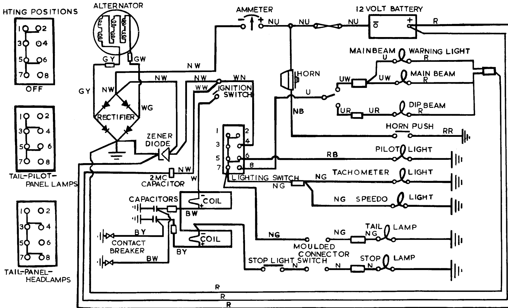
2MC CAPACITOR IGNITION SYSTEM
