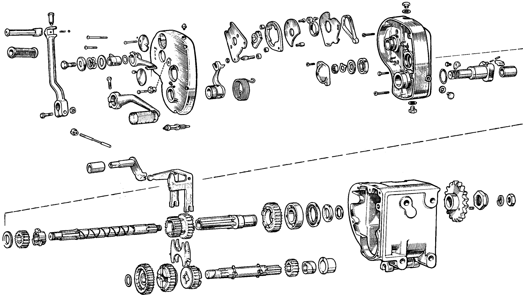
EXPLODED VIEW OF GEARBOX
